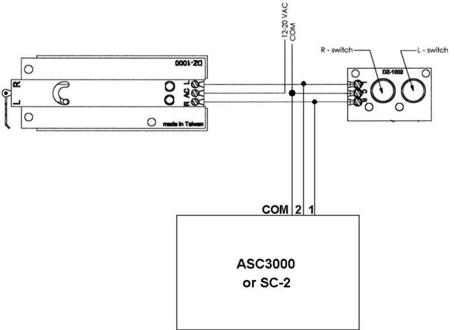
Power and Command control wiring as indicated by IC Controls.
